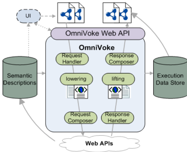
Figure 1. OmniVoke Architecture
