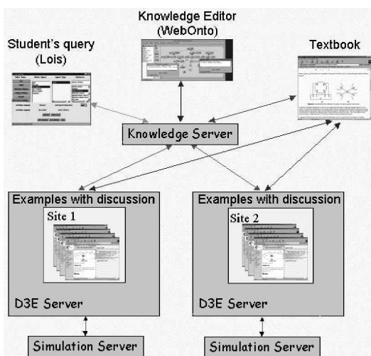
Figure 7. The RichODL architecture.
