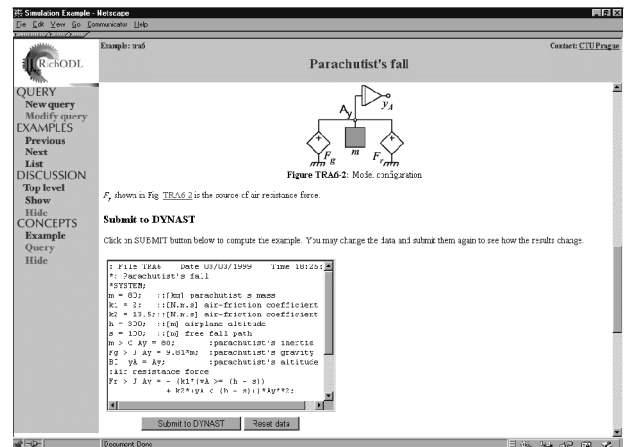
Figure 4. The solution to the Parachutist's fall problem described as a multipole diagram and Dynast code.
