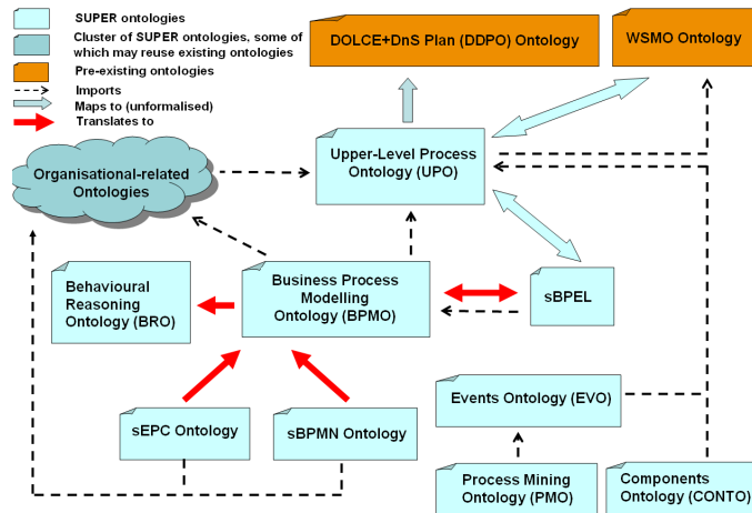
Fig. 1. SUPER Ontology Stack.
